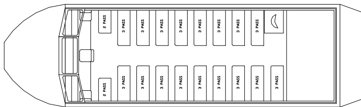
SEATING LAYOUT
